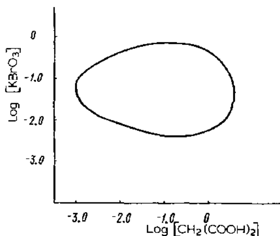
Fig. 4. The domain of existence of oscillations for the \text{KBrO}_3\text{-Ru}(\text{bipy})_3^{2+}\text{-CH}_2(\text{COOH})_2 system in the coordinates of \text{KBrO}_3 and \text{CH}_2(\text{COOH})_2 concentrations [45].
