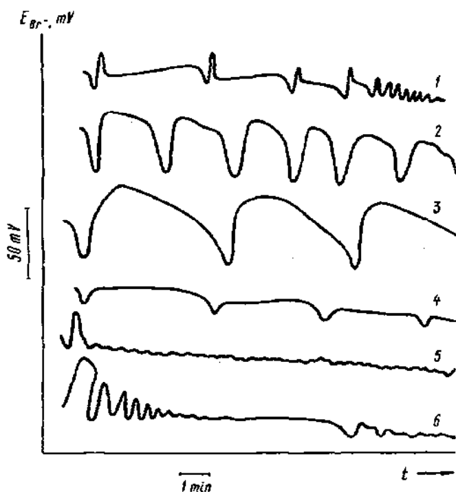
Fig. 8. Plots of the \text{Br}^- -selective electrode potential vs. time for \text{KBrO}_3 - \text{Ni}(\text{Me}_6[14]4,14 \text{ diene } \text{N}_4)^{2+} - \text{CH}_2(\text{COOH})_2 system under different concentration conditions [80].
