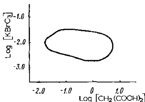
Fig. 3. The domain of existence of oscillations for the \text{KBrO}_3\text{-Fe}(\text{phen})_3^{2+}\text{-CH}_2(\text{COOH})_2 system in the coordinates of \text{KBrO}_3 and \text{CH}_2(\text{COOH})_2 concentrations [46].
